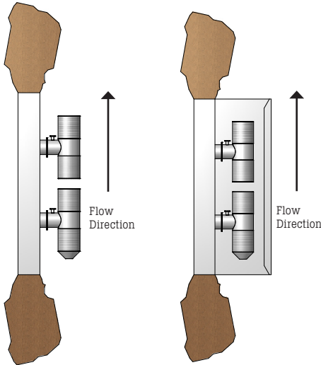
Typical Installation in faster moving, deeper rivers
